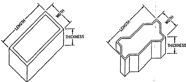
FIG. 1 Length, Width, and Thickness of Concrete Paving Units
